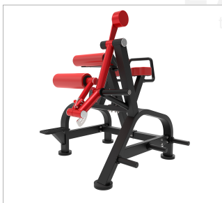
LP-034 Reverse Hyper Extension
